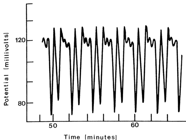
FIG. 1. Bromide ion electrode potential in the Belousov-Zhabotinsky reaction; reproduced from Hudson, Hart and Marinko, J. Chem. Phys. 71(4): 1601–1606, 1979.
