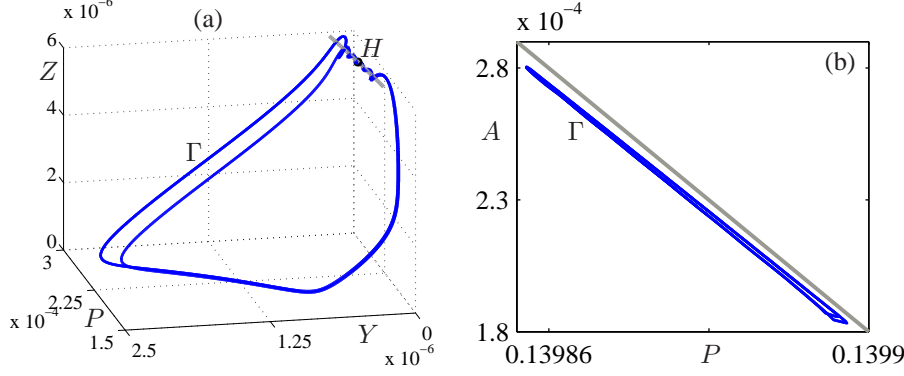
FIG. 31. (a) A three dimensional plot of the trajectory onto the space spanned by the coordinates (P, Y, Z) . A curve along the critical manifold is plotted as a grey line, and the black dot marks the location of a Hopf bifurcation in the fast subsystem. (b) The MMO is projected onto the coordinates A and P . The grey line is defined by 2A + P = 2A_0 and the ranges of A and P are [0.13985, 0.13991] and [0.00018, 0.0003] .
